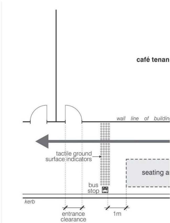
Figure 7 Clearances required around the outdoor dining area
